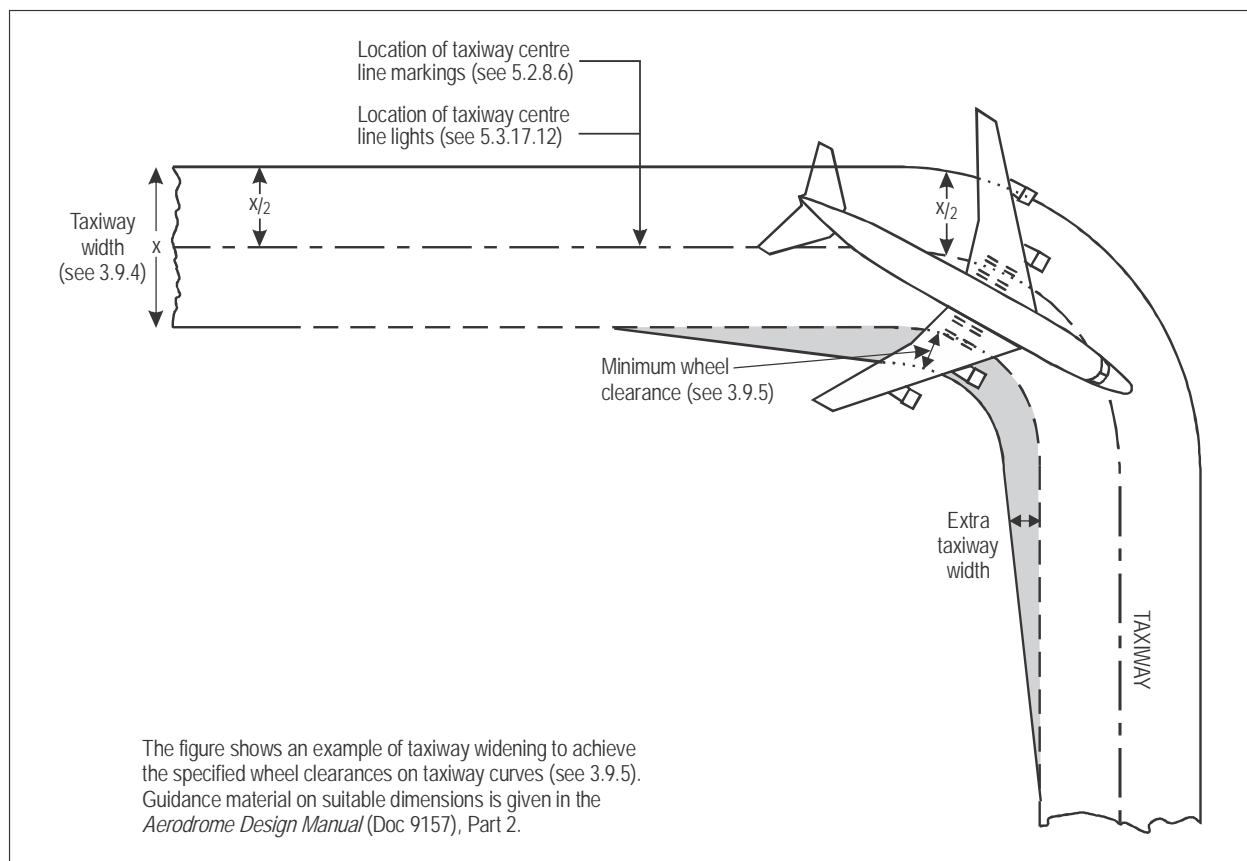
Figure 3-2. Taxiway curve
